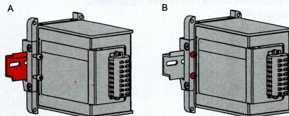
Fig. 9: C9900_U332_mounting on DIN rail
