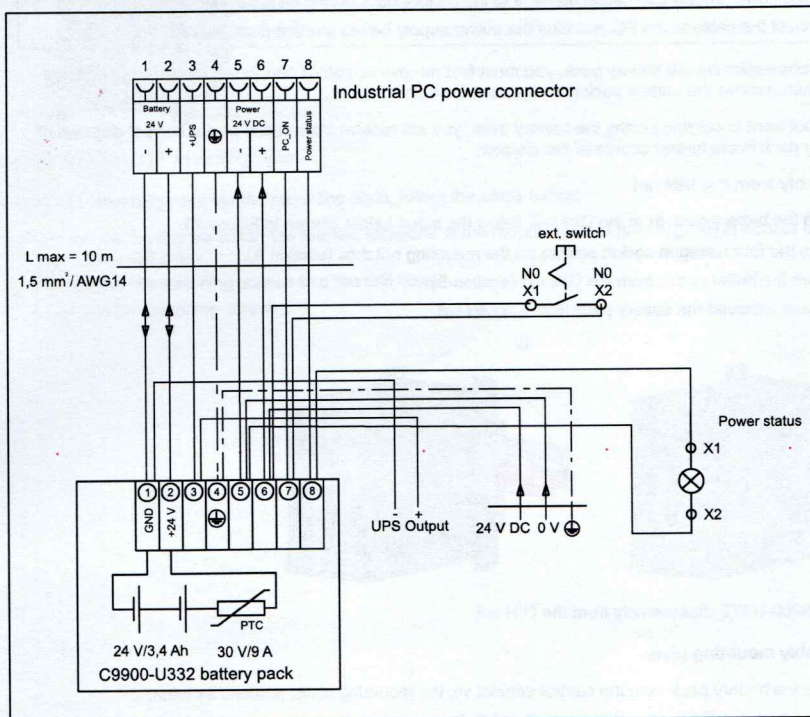
Fig. 13: C9900-U332_wiring diagram
